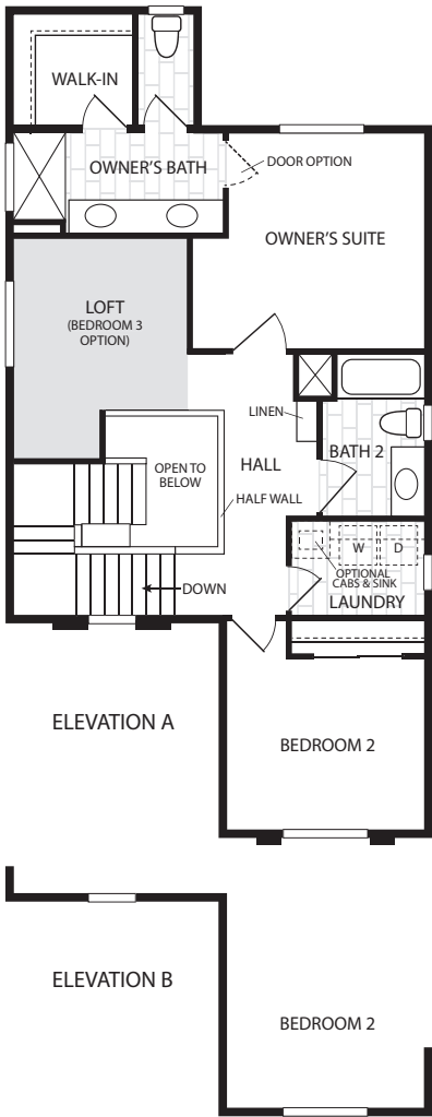
SECOND FLOOR
